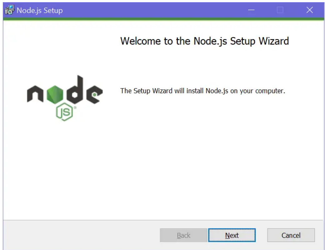
Node.js Installation
